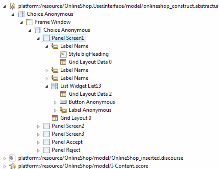
Figure 4.4: Abstract UI Description for Screen1
